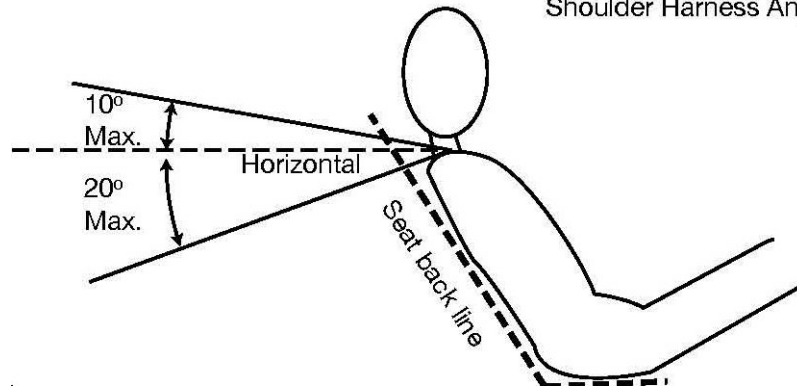
FIGURE 6 b Shoulder Harness Angle
