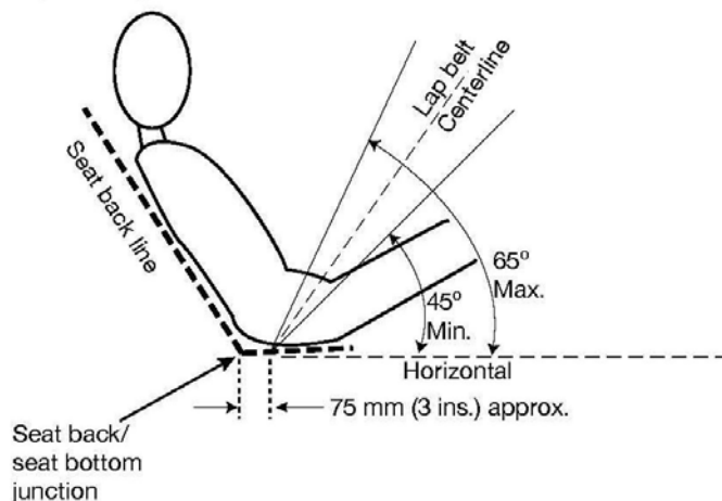
FIGURE 6 a Lap Belt Angle
